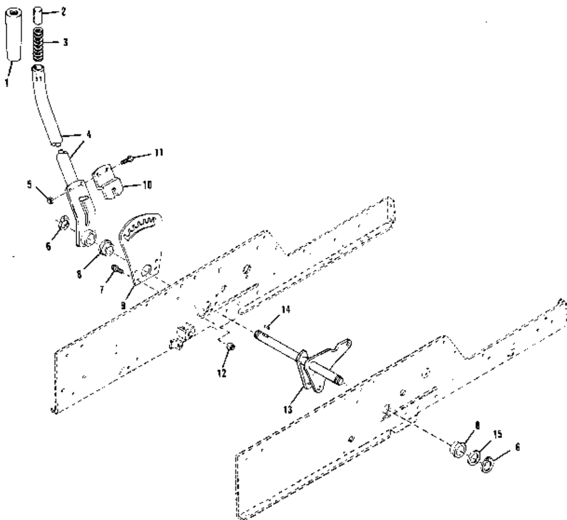
Figure 5. LIFT ASSEMBLY
