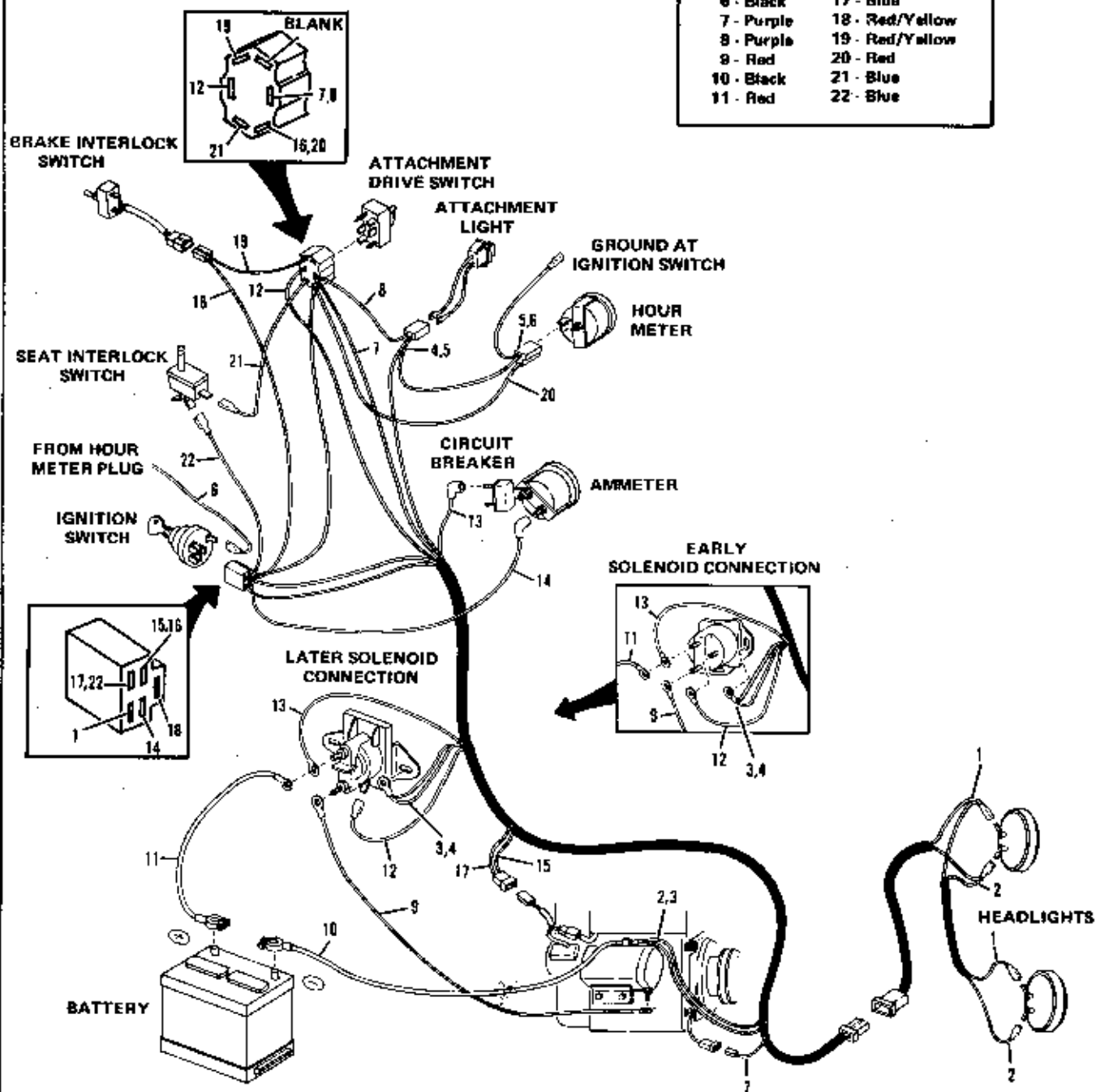
Figure 1 ELECTRICAL WIRING SYSTEM
